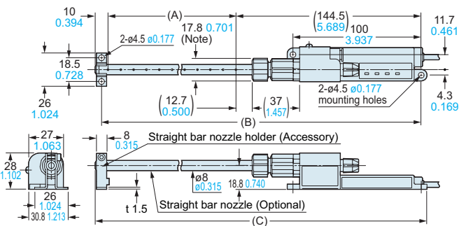
Mounting drawing with straight bar nozzle (ER-VAB□, Optional)
